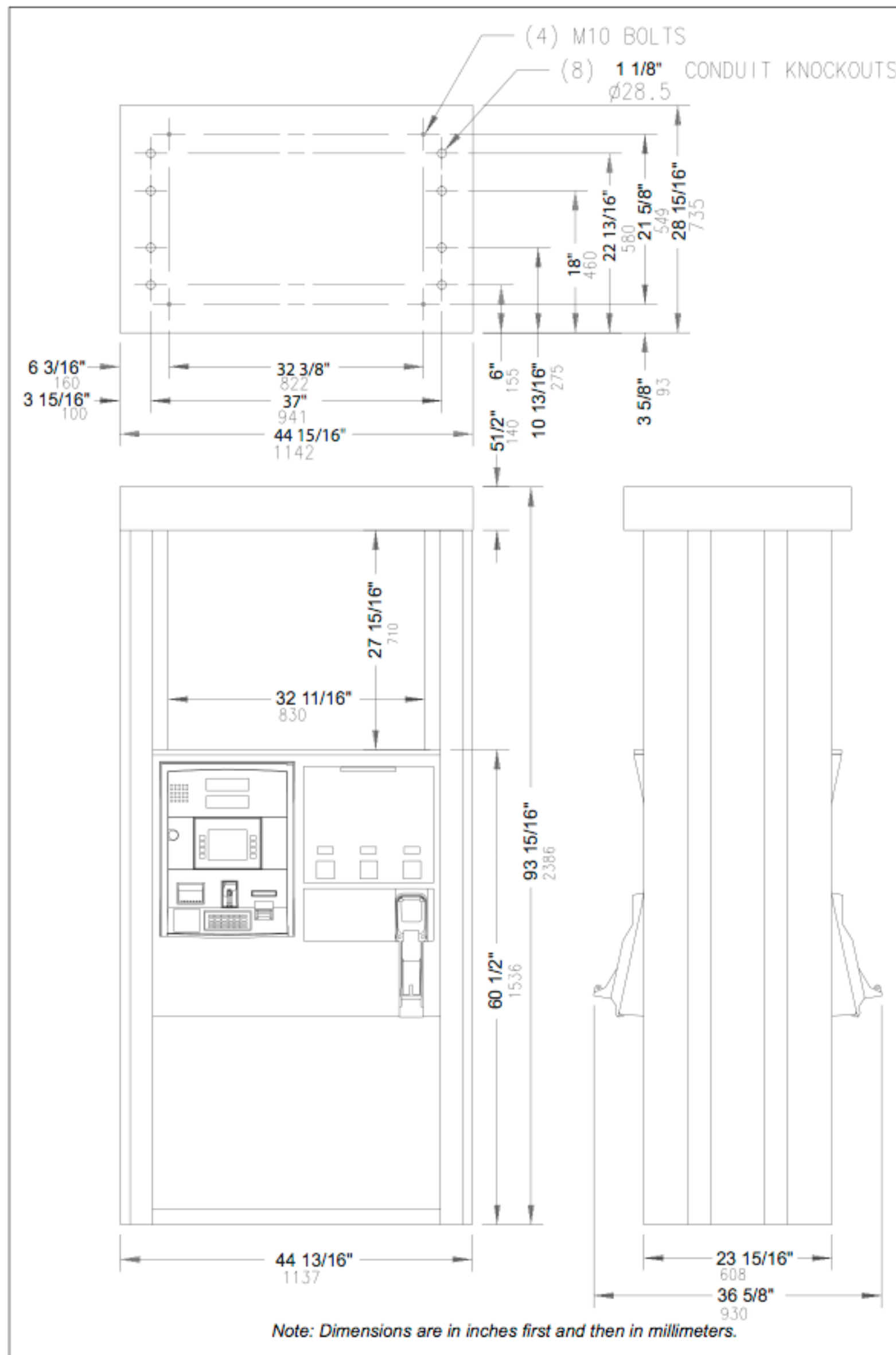
Figure A-9: Encore Elevation Diagram (Encore 550 with SMART Meter)
