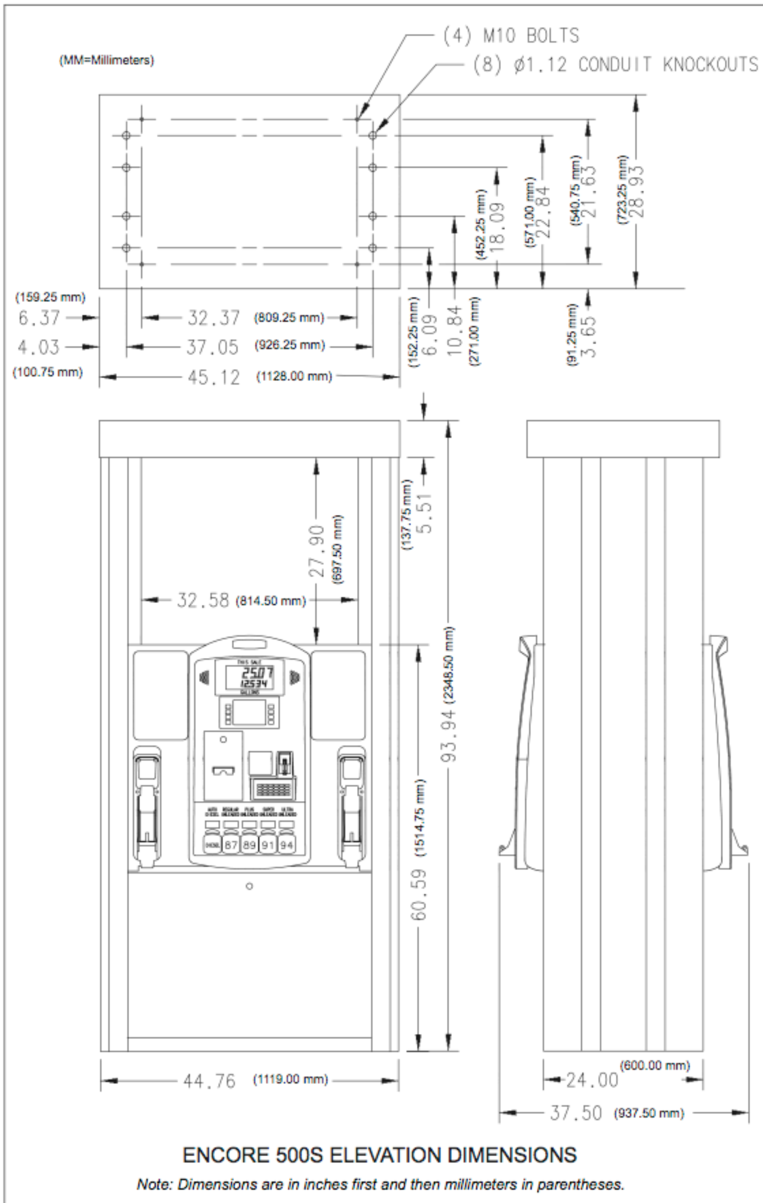
Figure A-10: Encore Elevation Diagram (Encore 500 S with SMART Meter)
